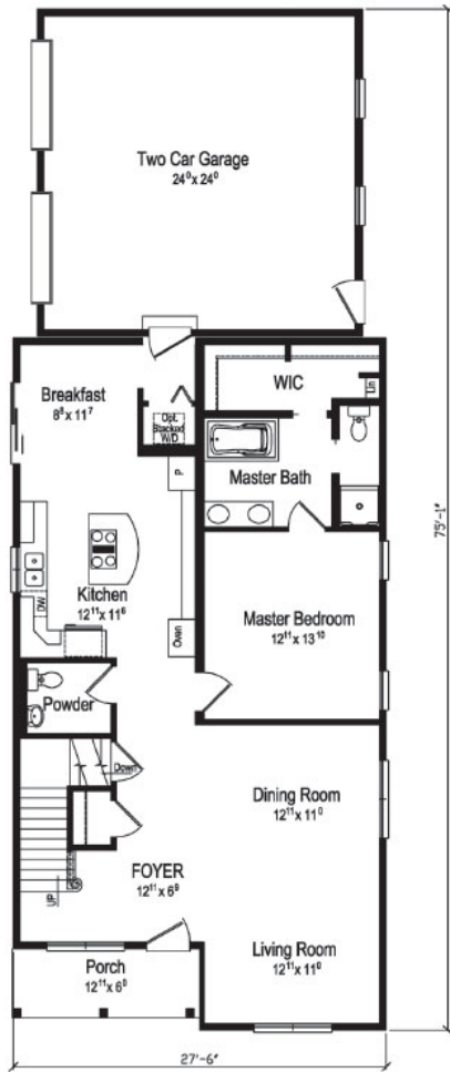
First Floor Plan Layout 9 foot Ceilings
