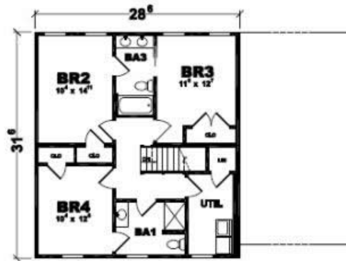
Second Floor Layout
