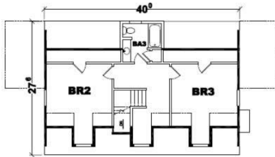
Proposed Second Floor Layout
